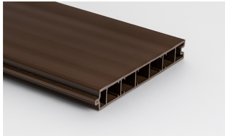
Ref. 015083WP Panel de 250x35 mm
